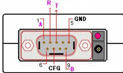
RS-232/485/422
